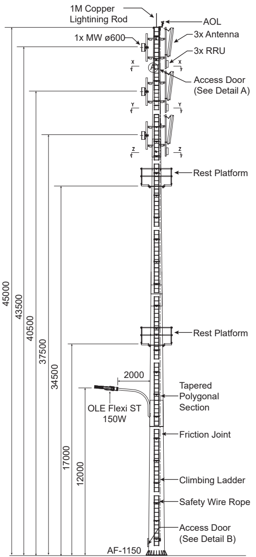
45M Monopole 3 Station
