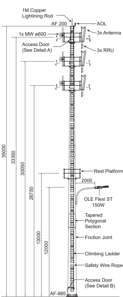
35M Monopole 3 Station
