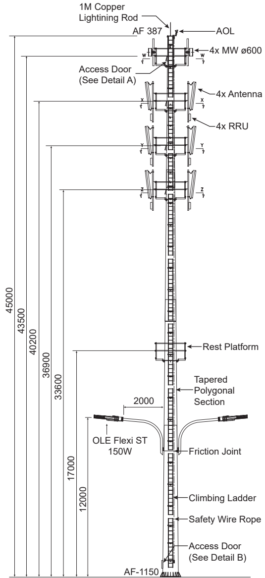
45M Monopole 4 Station
