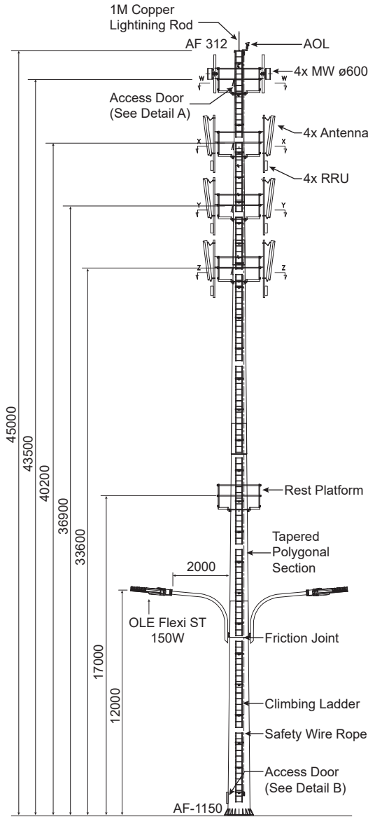
45M Monopole 4 Station
