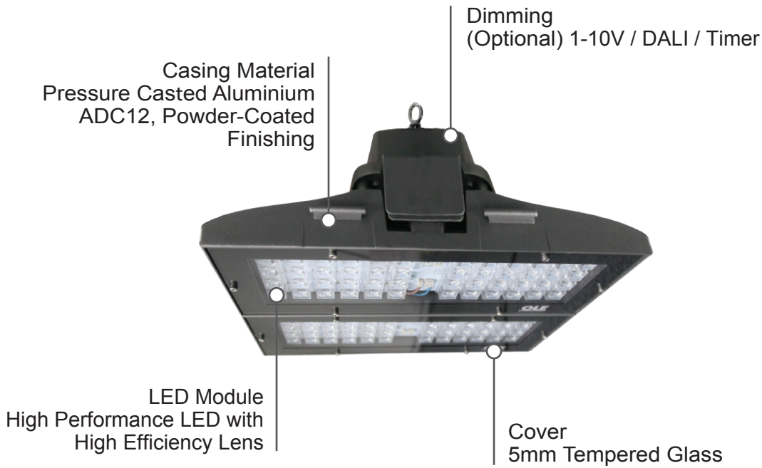
Ring Outfit Mounting
