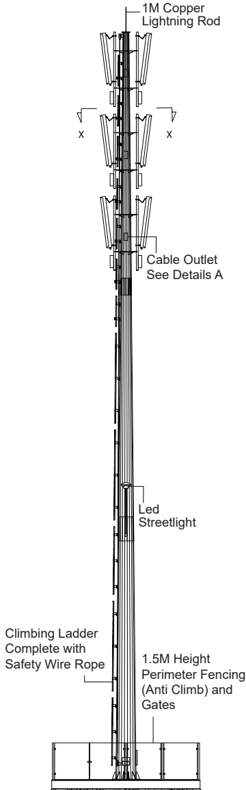
Side View
