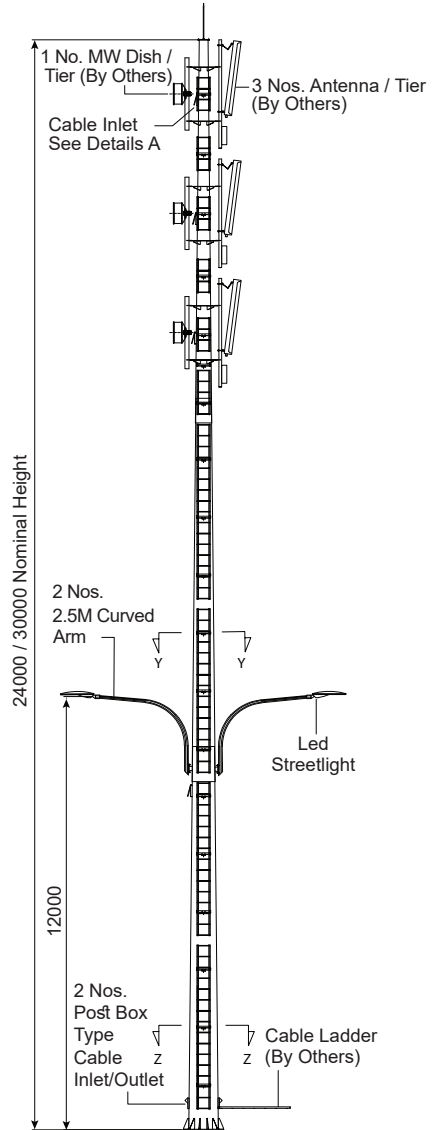
Front View
