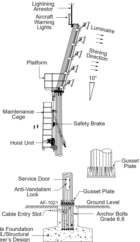
Side Elevation
