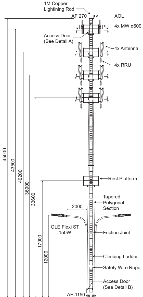
45M Monopole 4 Station
