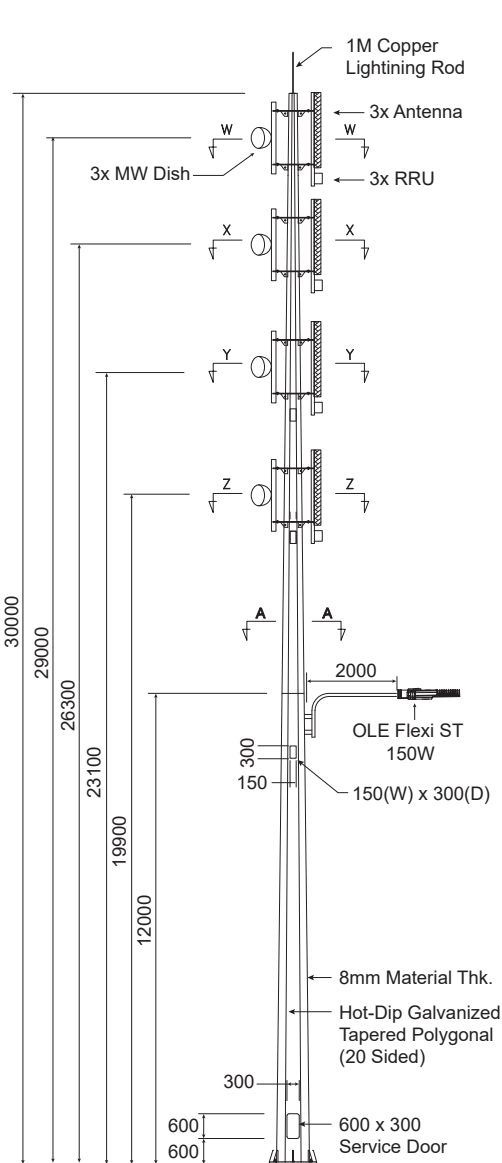
30M Monopole 4 Station
