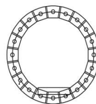
Base Flange Stiffened with Gussets
