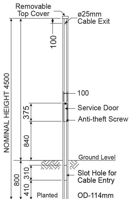
Planted Type
