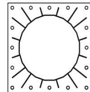
Base Flange Stiffened with Gussets
