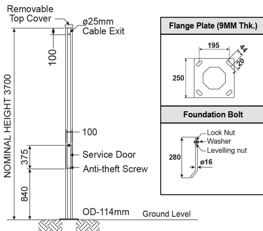
Flange Type
