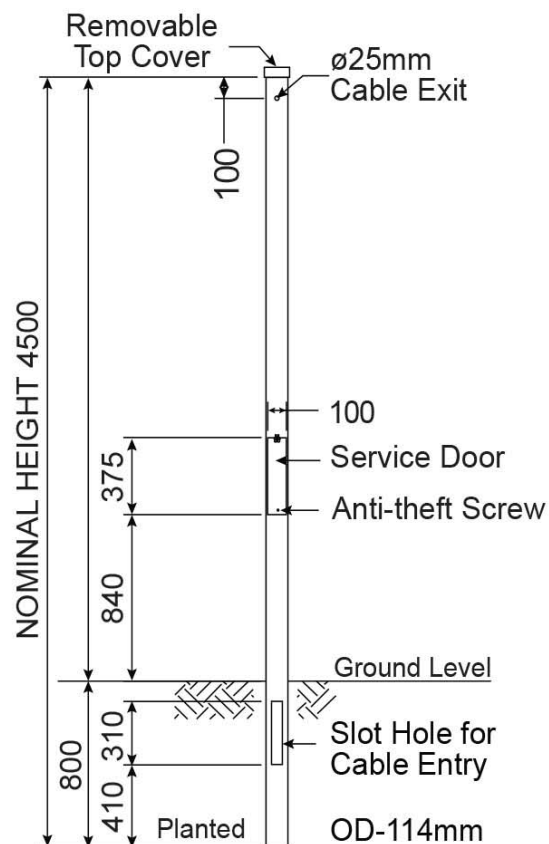
Planted Type
