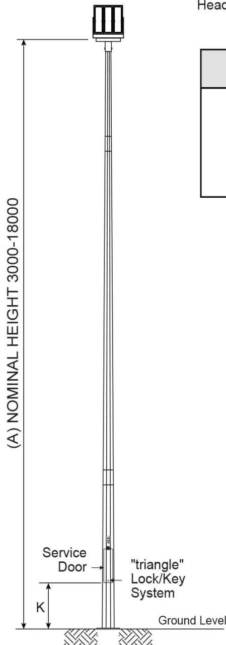
2 or 3 Section Column based on Height
