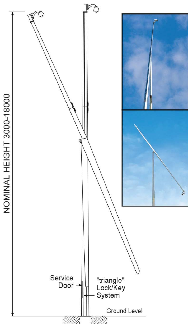
Mid-Hinged Pole
