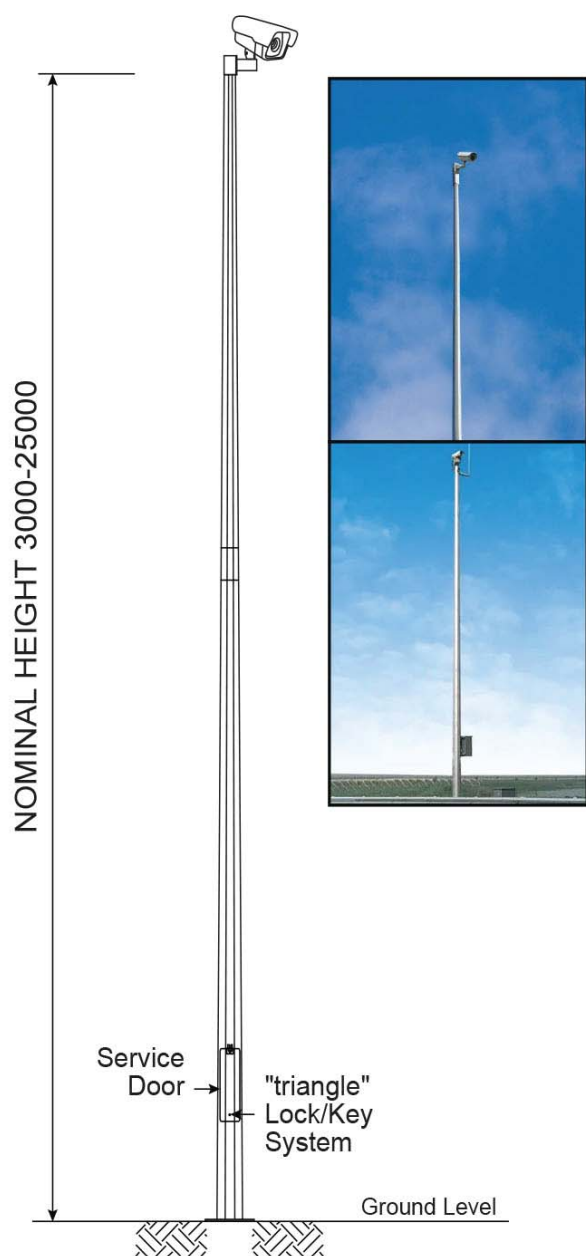
Octagonal Pole
