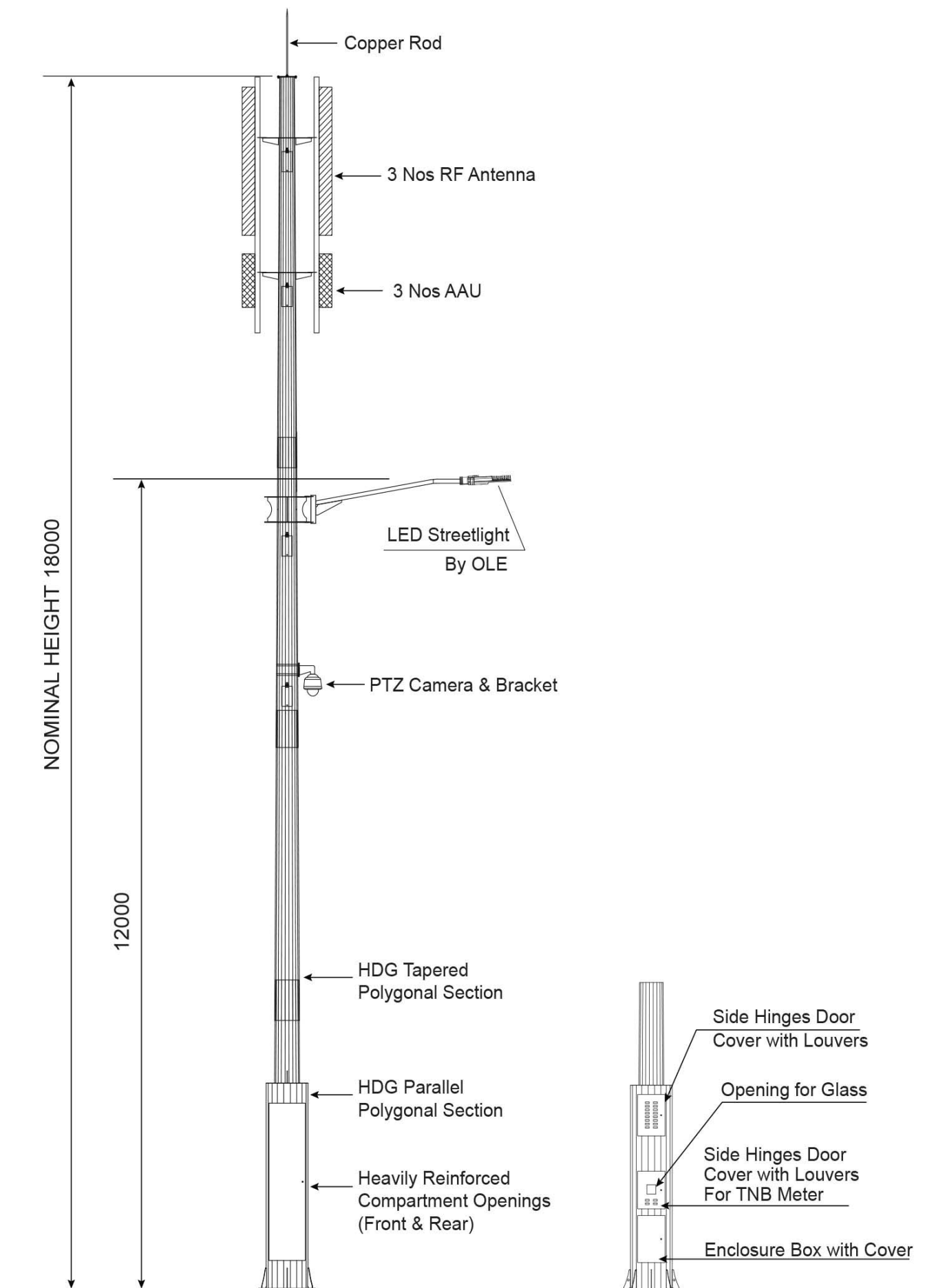
Rear View
