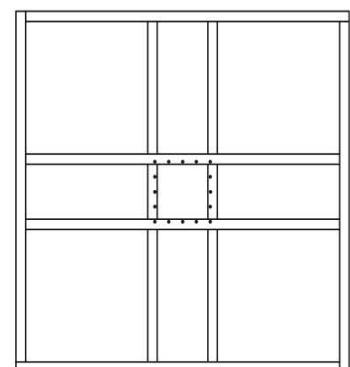
Counterweight Base Filled with Crusher Run and Gravel Stones Plan View
