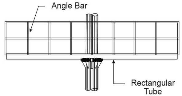
Platform Elevation
