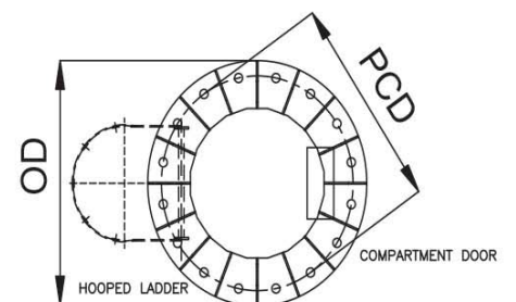
Base Flange Stiffened with Gusset
