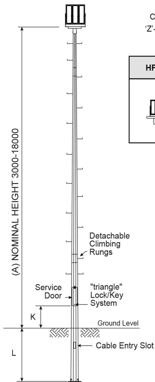
2 or 3 Section Column based on Height
