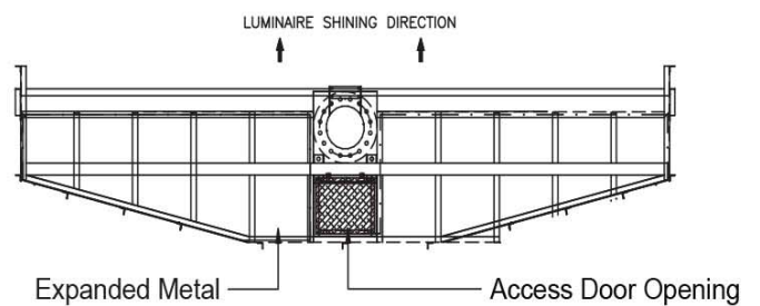
Platform Plan
