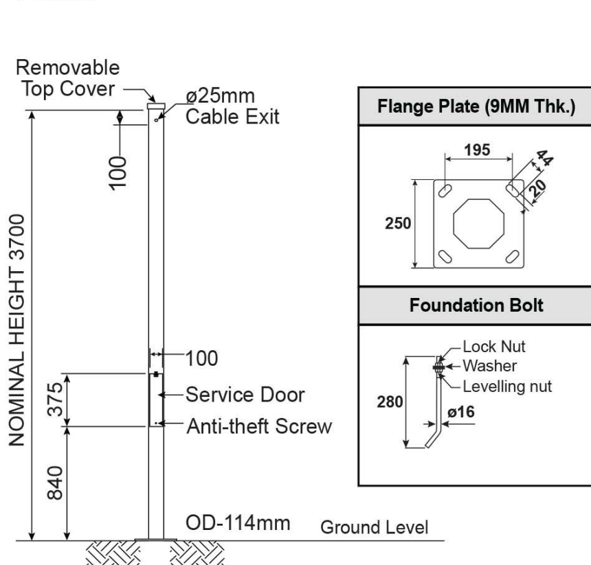
Flange Type
