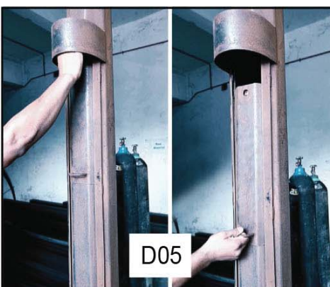
Sliding Service Door c/w Locking Guard & Handle
