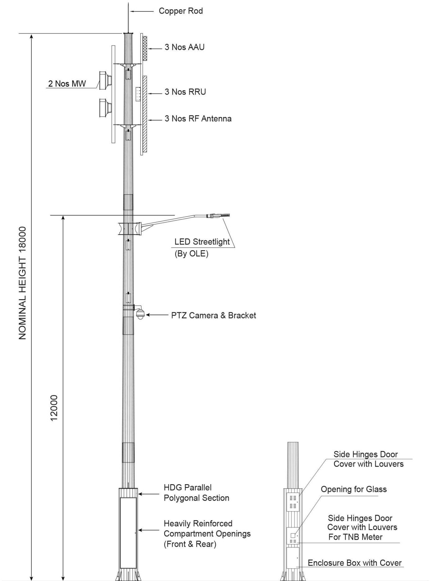
Rear View
