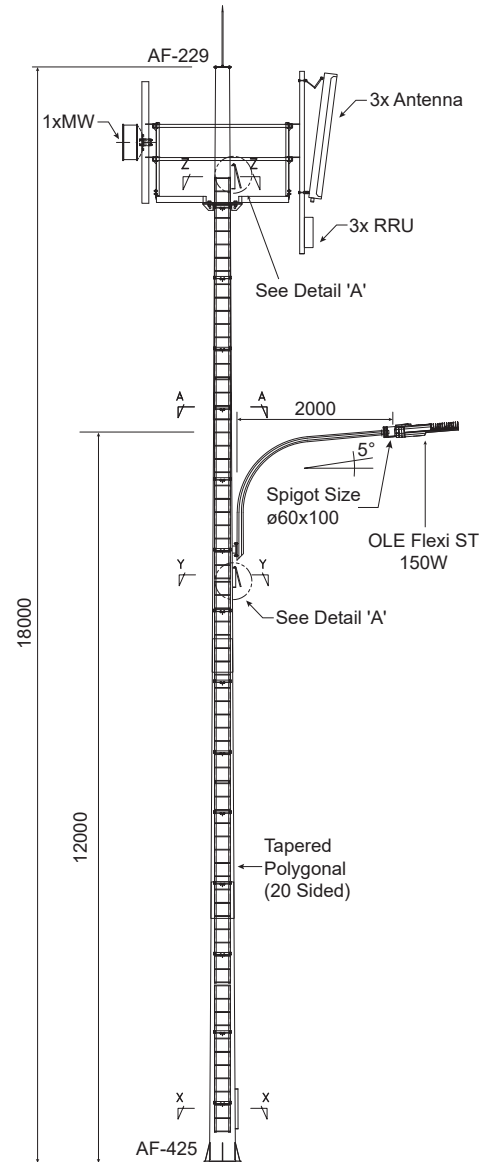
18M Monopole 1 Station
