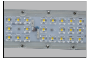
LED Module
